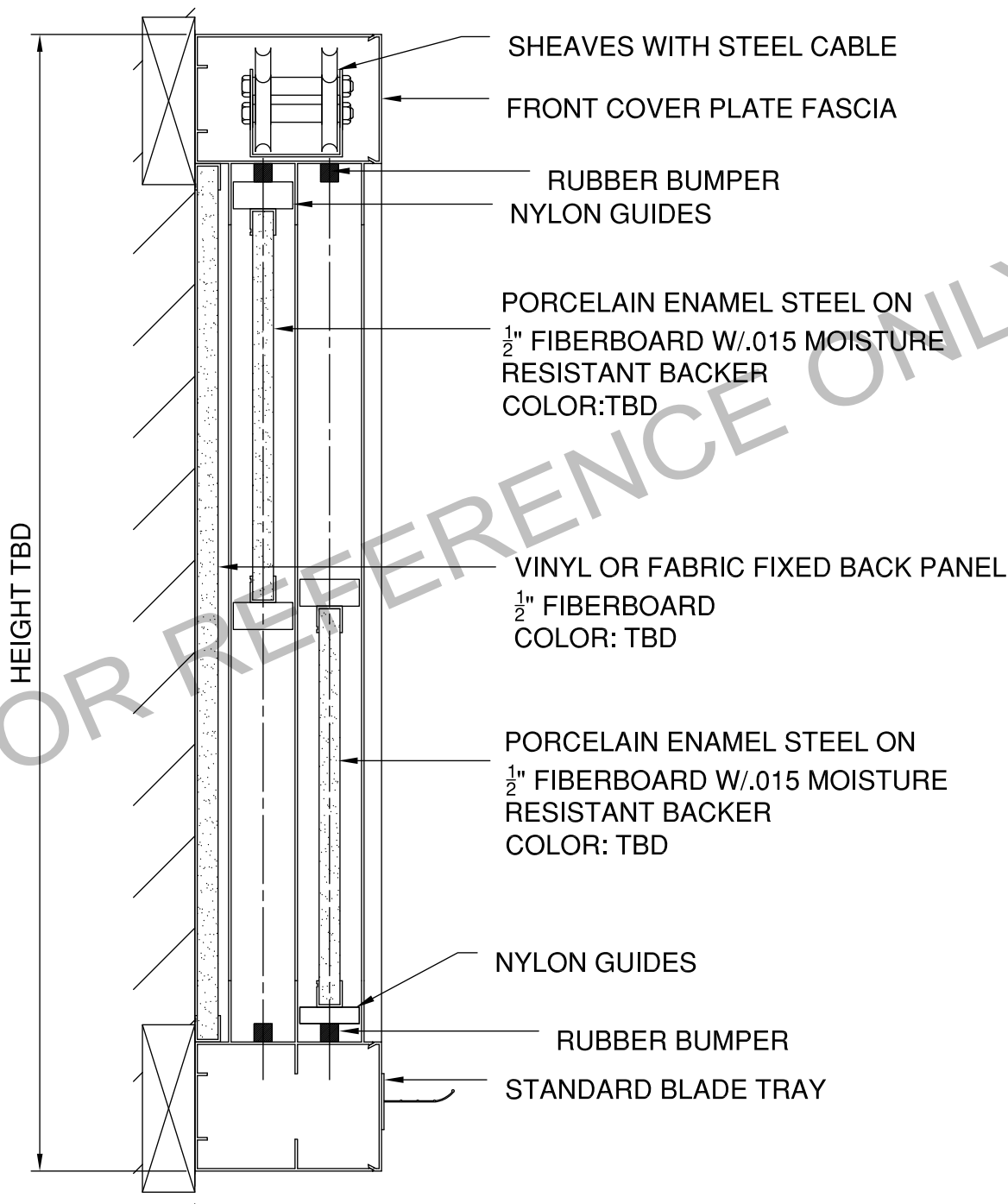
Side Detail
