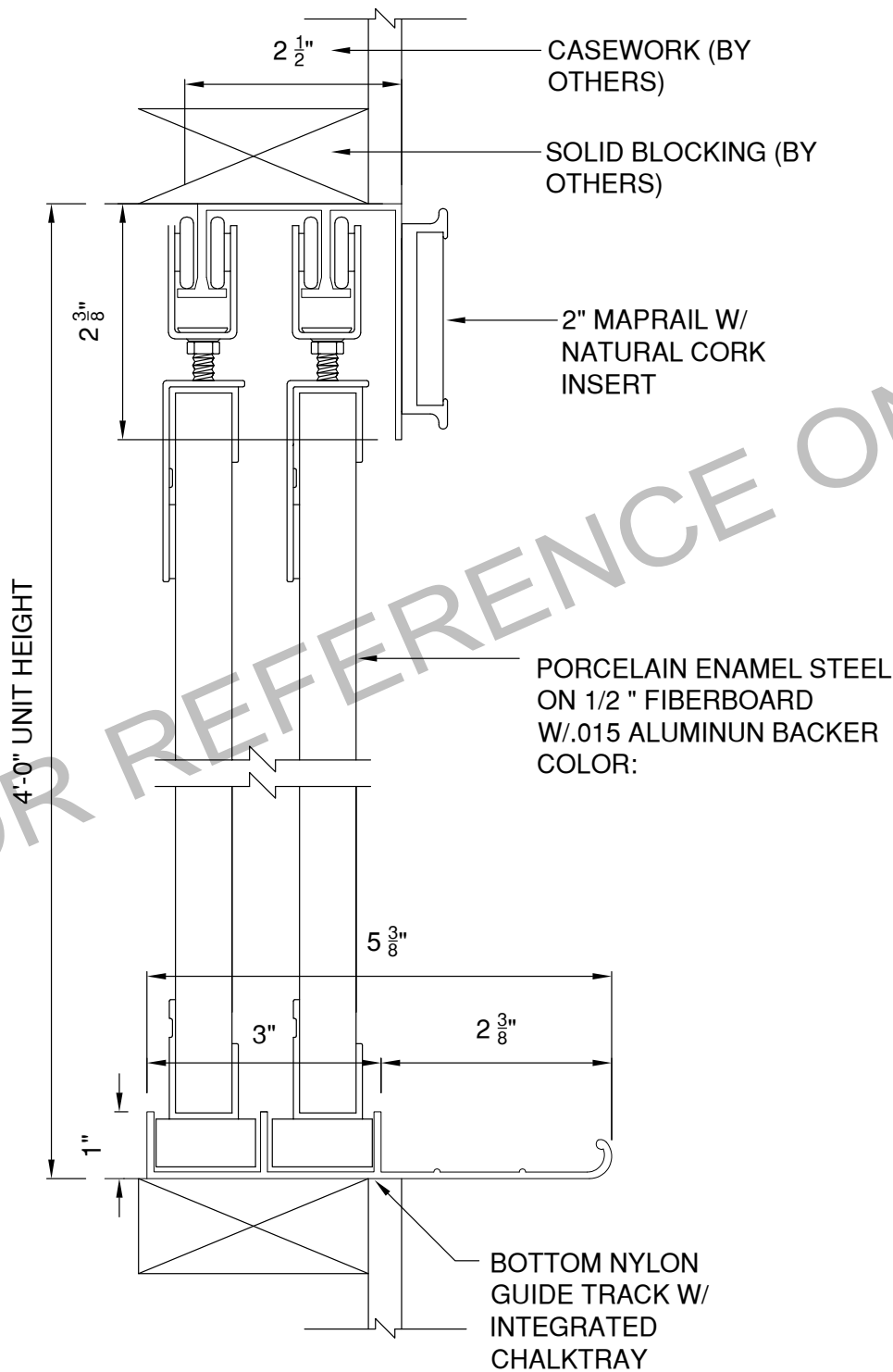
Side Detail
