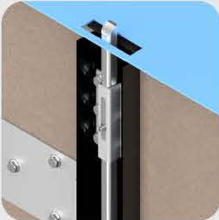
KNOX TABLE LOCK
